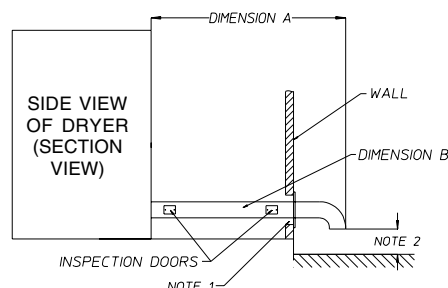
HORIZONTAL DUCTING
