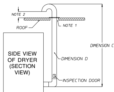
VERTICAL DUCTING
