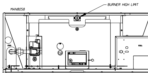
GAS DRYER FRONT VIEW – CONTROL DOOR OPEN
