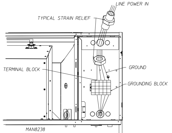
REAR VIEW WITH ELECTRIC HEAT – GUARDS AND COVERS REMOVED
