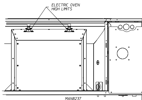
ELECTRIC DRYER REAR VIEW – TOP BACK GUARD REMOVED
